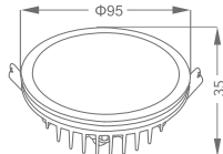
16W Cutting size / \Phi 95
