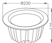
80W Cutting size Φ210
