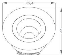
5W Cutting size Φ70
