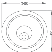
7W Cutting size Φ80
