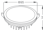
9W Cutting size / \Phi 75
