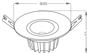
7W Cutting size \Phi 75
