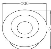
50W Cutting size \Phi 30
