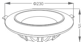
32W Cutting size Φ185-190
