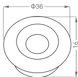
12W Cutting size \Phi 30
